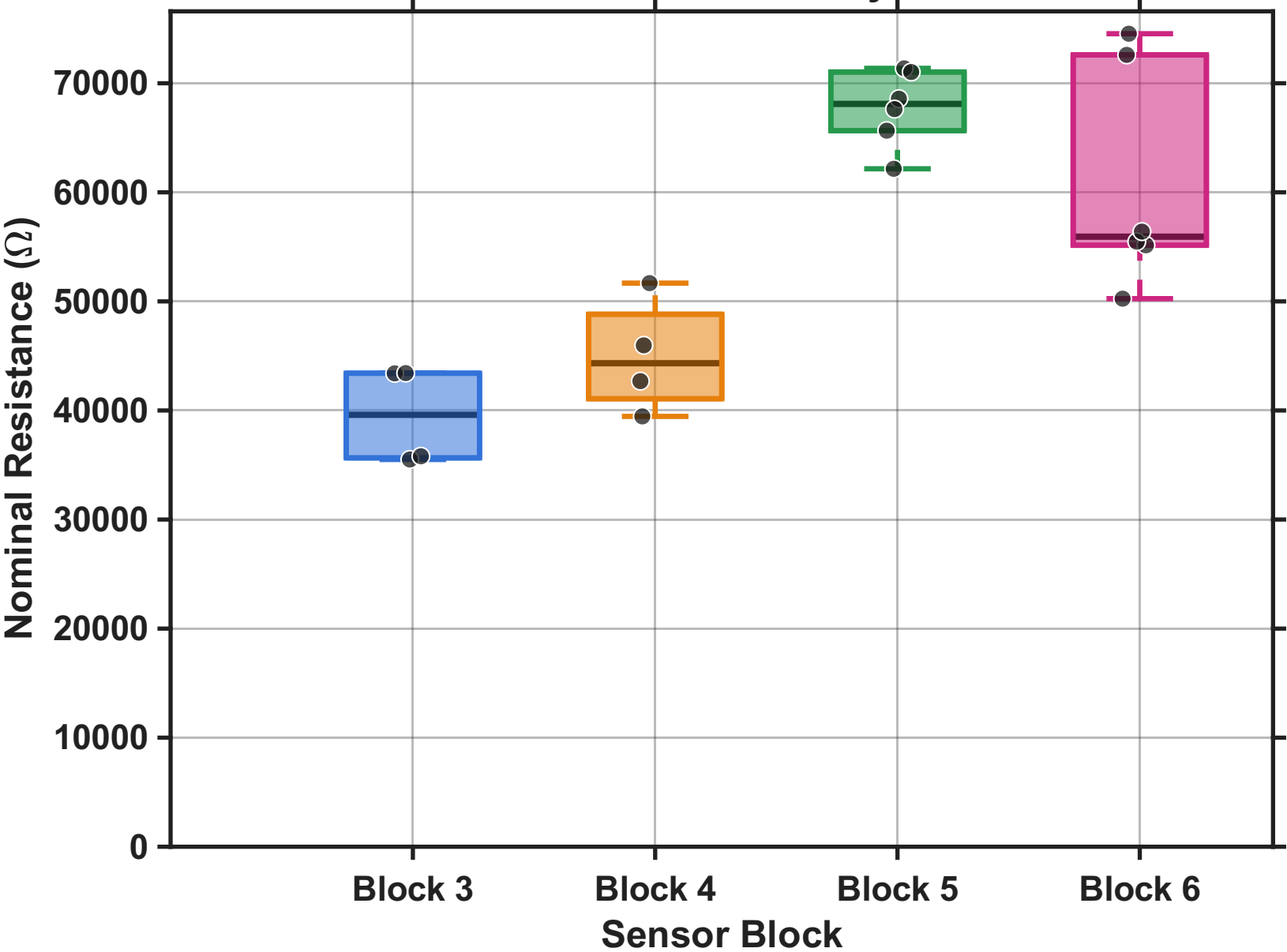
Nominal Resistance Variation by Sensor Block
